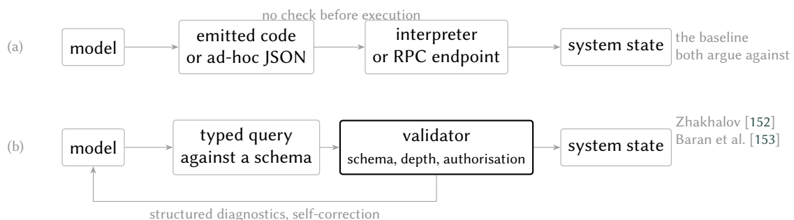
Figure 33: Free-form code-generating agency (a) against schema-constrained agency (b). In (a) the model’s output reaches an interpreter or endpoint with no machine-checkable contract in between, so the action space is whatever the runtime permits. In (b) the action is a typed query, a validator outside the model accepts or rejects it before execution, and rejection returns structured diagnostics the model can act on. The measurable benefit is structural reliability and a bounded attack surface; §9.3 gives the DOI-verified evidence that constraining generation can also cost reasoning quality, and why constraining the action rather than the deliberation sits on the favourable side of that trade.
