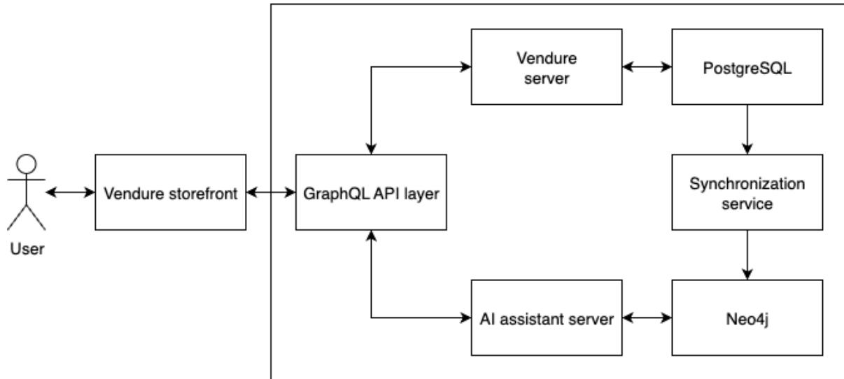
Figure 3: Architecture overview.
