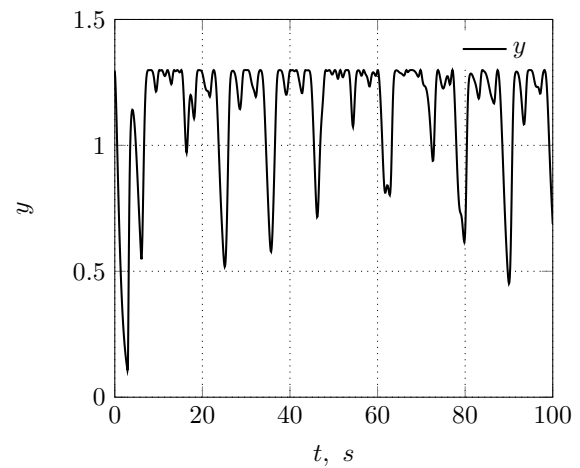
Figure 12: y , K = 1 .
