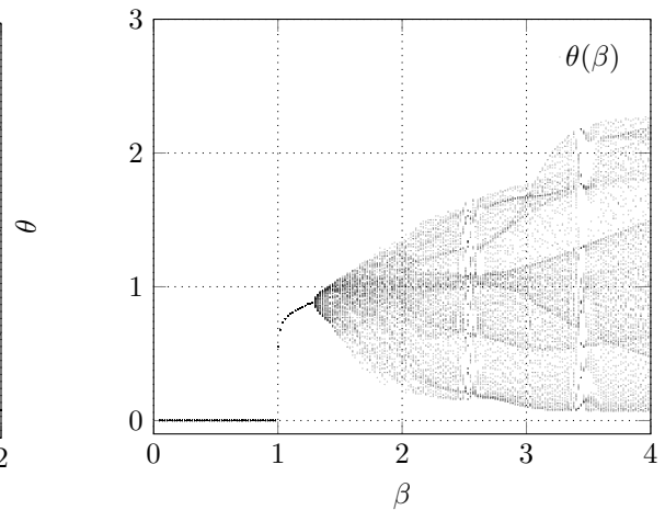
Figure 30: \beta = var.
