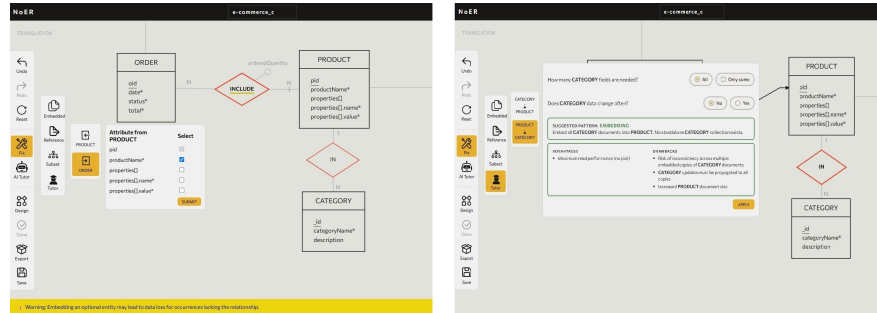
Figure 2: Examples of document-oriented relationship translation patterns supported by NoER, including extended referencing and embedding when using the Guided Pattern Selection functionality.
