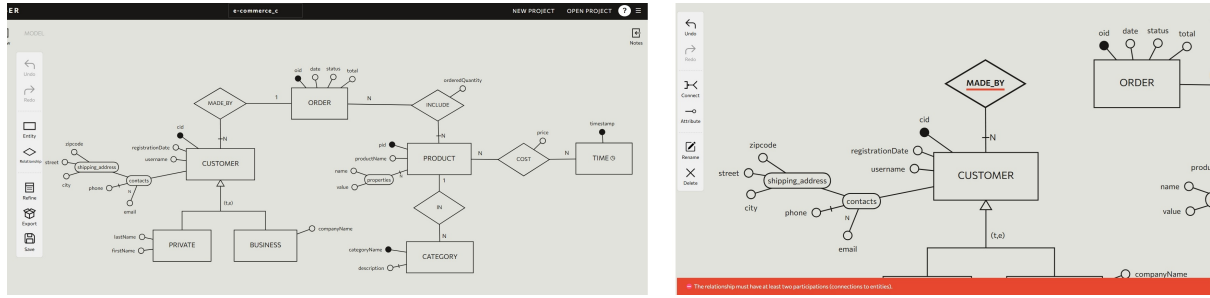
Figure 1: ER d conceptual schema of the running "e-commerce" use case created. The figure shows an example of detected error during conceptual modeling when a relationship is missing a connection.
