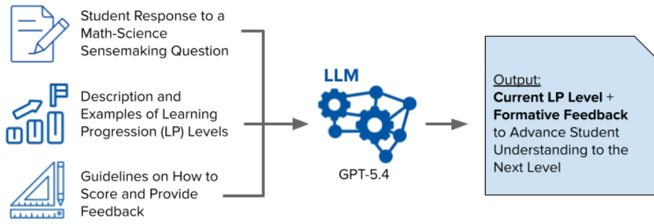
Figure 1: Overview of the LLM-based scoring and feedback generation workflow
