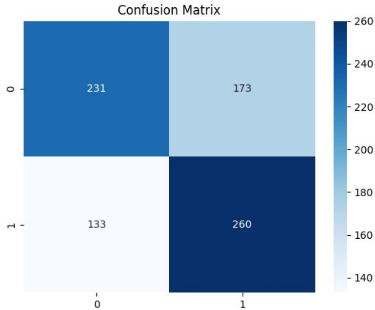
Figure 1: Confusion matrix on the validation set (0 = not sexist, 1 = sexist).
