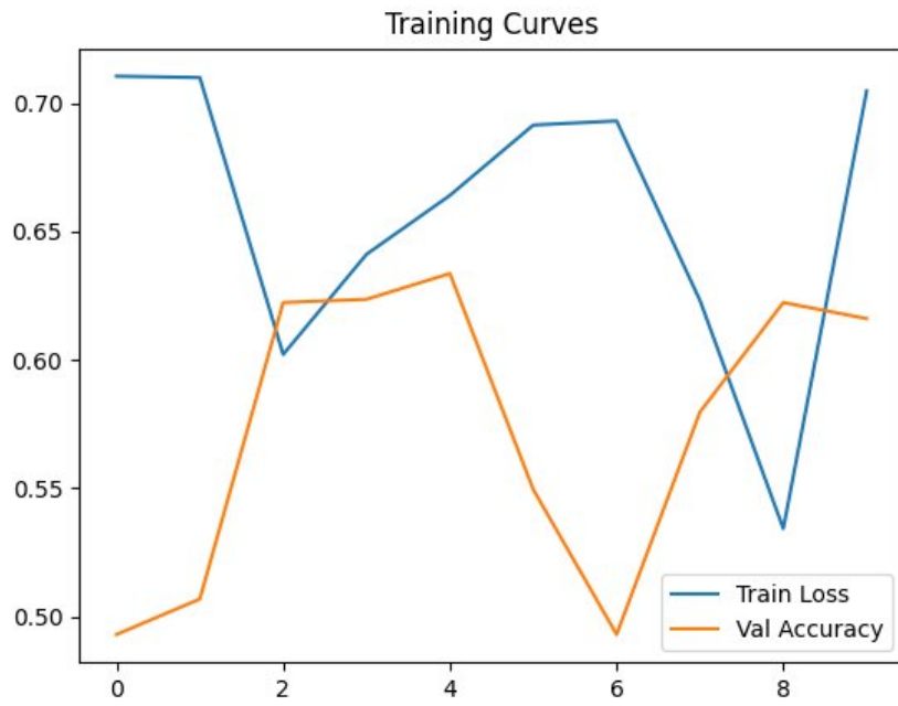
Figure 3: Training loss and validation accuracy over 10 epochs.
