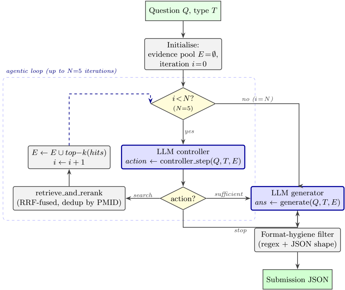
Figure 2: The agentic control loop. The LLM controller chooses one of three actions per iteration: search (issue a reformulated query, ingest top- k RRF-fused hits, increment i , loop), sufficient (terminate and proceed to generation), or stop (terminate without an answer). A hard cap of N=5 iterations guarantees the loop halts even if the controller never declares sufficiency.
