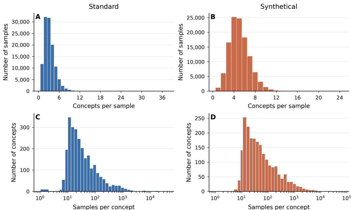
Figure 2: Distribution of CUI annotations before rare-label filtering. The upper panels show the number of assigned CUI concepts per training sample, and the lower panels show the number of training samples assigned to each CUI concept. Both standard and synthetical splits exhibit long-tailed CUI distributions, motivating the removal of labels that appear fewer than 20 times.
