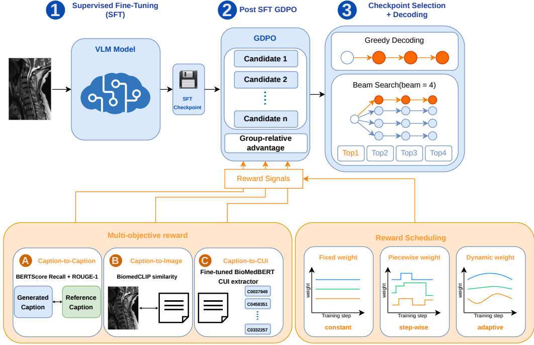
Figure 1: Overview of the proposed GDPO-based medical image captioning pipeline. After supervised fine-tuning, the model is optimized with post-SFT GDPO using multi-objective reward signals. The reward function is organized around three alignment axes: caption-to-caption alignment, caption-to-image alignment, and caption-to-CUI alignment. Reward scheduling controls the relative contribution of the reward components during GDPO training, and the final system uses checkpoint selection followed by greedy or beam-search decoding.; CC BY[Hongo et al. (2018)]
