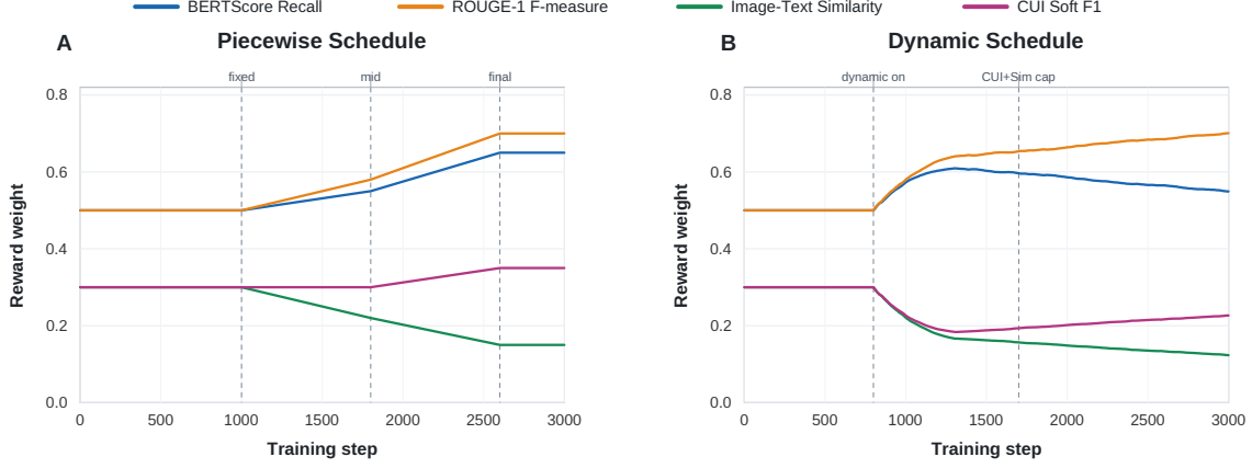
Figure 3: Reward-weight trajectories for the piecewise and dynamic scheduling strategies. The piecewise schedule follows predefined interpolation intervals, while the dynamic schedule updates weights online using advantage-alignment statistics under predefined constraints. Despite different update mechanisms, both schedules shift weight toward caption-to-caption rewards and reduce the image-text similarity weight during later training.
