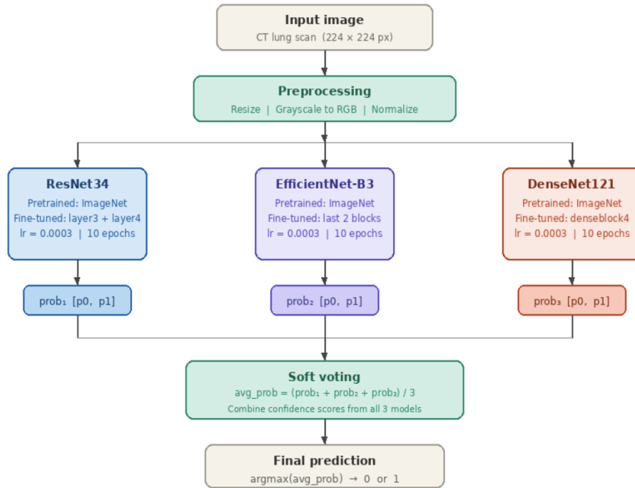
Figure 1: Proposed ensemble architecture using soft voting.
