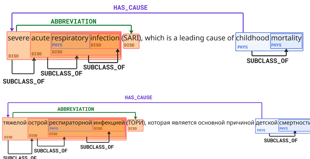
Figure 1: Example of nested named entity relations in the BioNNE-R dataset.
