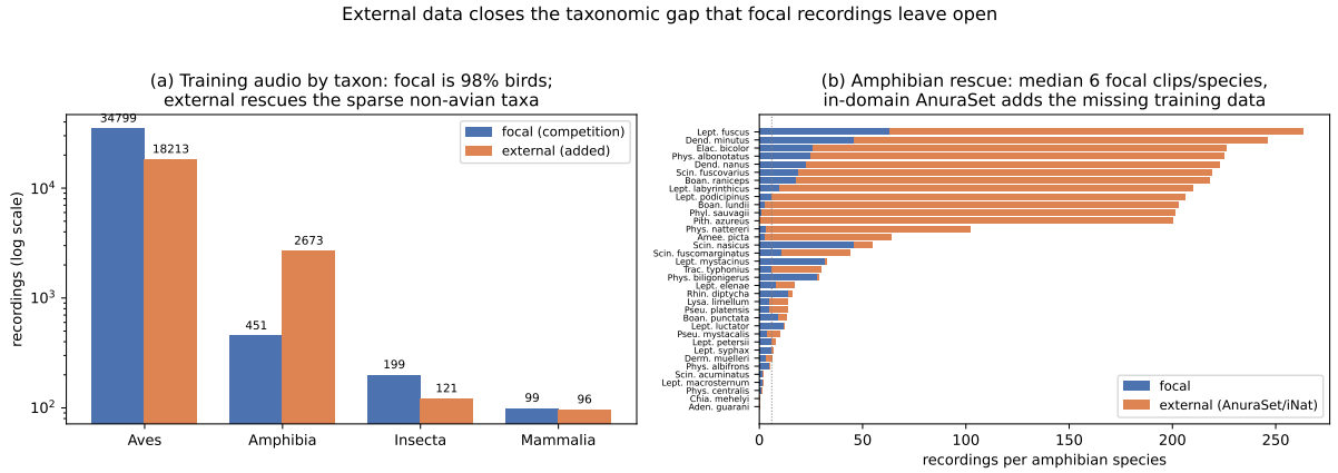
Figure 3: Why external data helped. (a) Training audio by taxon (log scale): focal recordings are 98% birds; external data rescues the sparse non-avian taxa. (b) Per-amphibian-species rescue: most species sit at or below the focal median (dotted line); in-domain AnuraSet / iNaturalist data lifts them by an order of magnitude. Insects cannot be rescued: most are unidentified sound types with no external counterpart.
