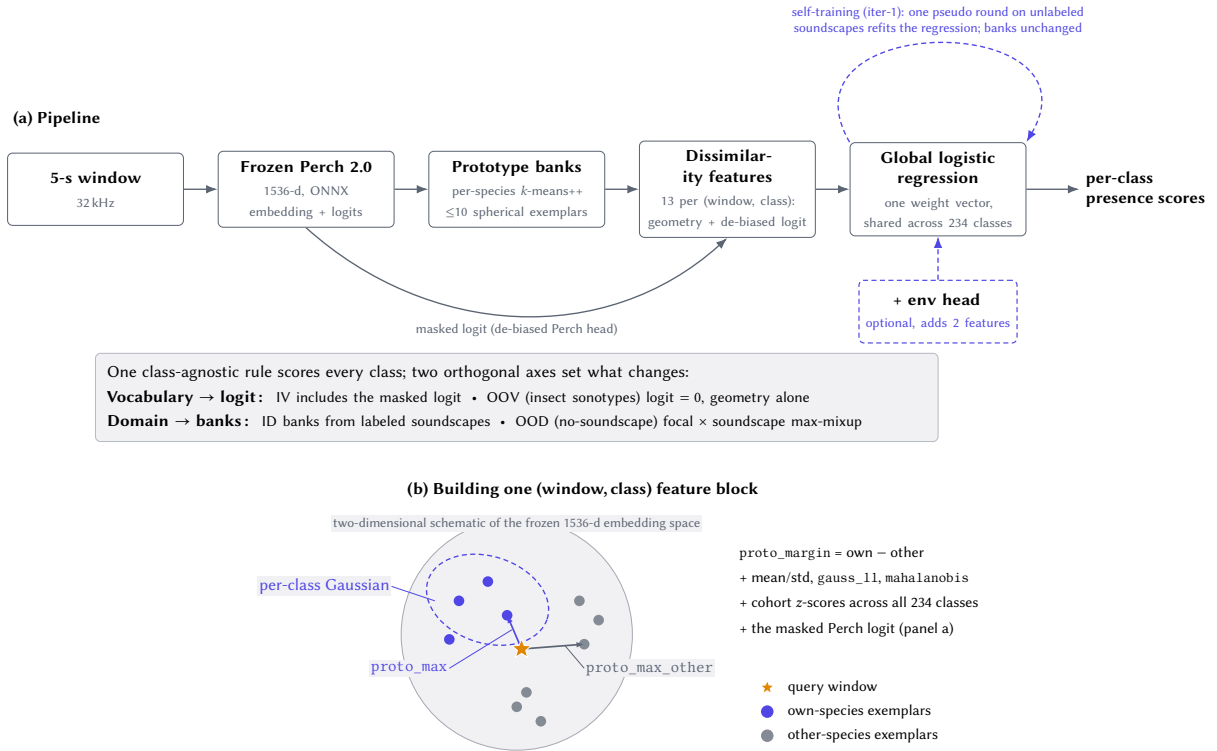
Figure 1: The GREBE pipeline. (a) A 5-s window is embedded once by a frozen Perch 2.0 model; per-species prototype banks ( k -means++ exemplars, at most ten per class, scored against spherical-mean centroids) and the model’s own masked, de-biased logit yield 13 class-relative dissimilarity features per (window, class). A single global logistic regression, one weight vector shared across all 234 classes, maps those features to per-class presence scores. One class-agnostic rule scores every class; two orthogonal axes set what changes per class. Vocabulary, whether a class is in-vocabulary (IV) or out-of-vocabulary (OOV), governs whether the Perch logit is available; domain, whether it is in-domain (ID) or out-of-domain (OOD), governs how the banks are built (labeled soundscapes versus a focal-by-soundscape max-mixup for the no-soundscape species). Self-training adds one pseudo round that refits only the regression, leaving the banks unchanged (Section 4.6); the environmental head is an optional extension that appends two features (Section 4.7). (b) The Dissimilarity-features step for a single query window. Each feature is a relative geometric quantity, not a thresholded decision: the cosine similarity to the nearest own-species exemplar (proto_max), the similarity to the nearest other-species exemplar (proto_max_other), their margin, the mean and spread over the class’s own exemplars, a per-class Gaussian (gauss_11, mahalanobis), and cohort z-scores that rank each score across all 234 classes. The same shared classifier reads this feature block for every class, so a rare species is handled by the identical rule with fewer exemplars, never by a species-specific similarity cutoff.
