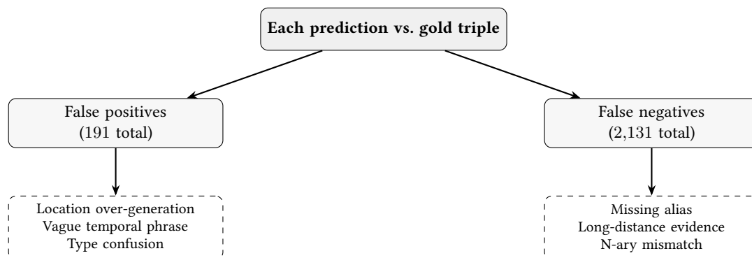
Figure 5: Taxonomy of the six residual error modes. The three false-positive modes are addressable with sharper post-processing; the three false-negative modes stem from the recall ceiling and the alias-set evaluation protocol.
