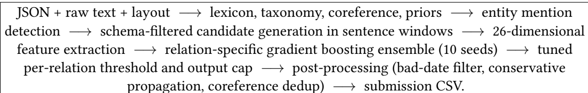
Figure 3: Overview of the proposed pipeline.
