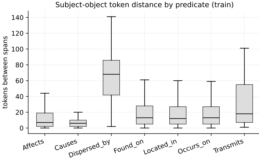
Figure 2: Subject-object token distance for gold text-bound relations in the train split, by predicate. Outliers are omitted.
