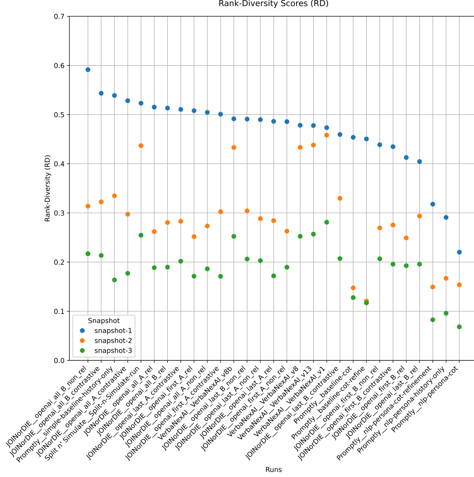
Figure 3: Similarity to the Ground-Truth Next Query evaluated using Rank-Diversity Score across sessions.
