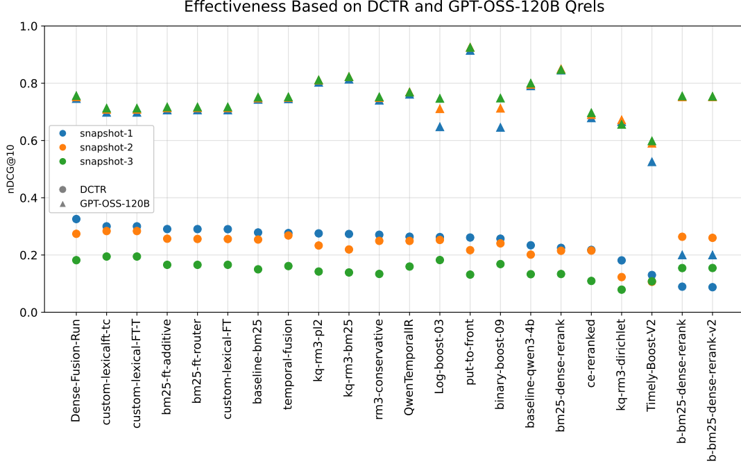
Figure 1: Effectiveness measured by nDCG@10 across all approaches and test snapshots using the DCTR qrels (opaque) and the synthetic relevance labels generated with GPT-OSS-120b (faded).
