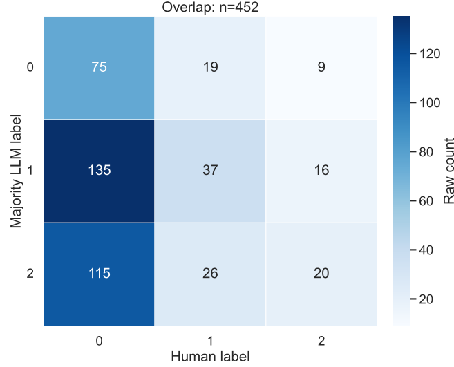
Figure 2: The confusion matrix of relevance judgments from large language models (the majority vote of all LLMs with all topic formalizations) and the human labels derived from click logs over the three snapshots.
