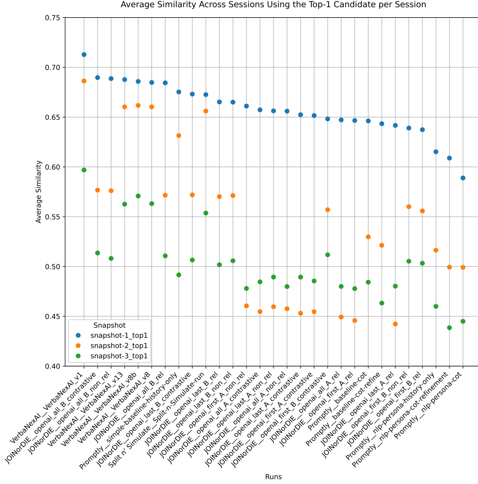
Figure 4: Cosine Similarity of the Top-1 Candidate per Session.
