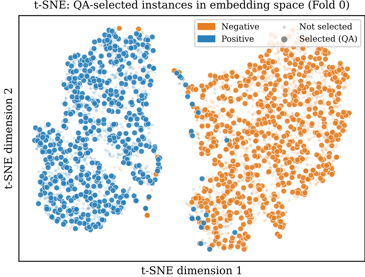
Figure 2: t-SNE [10] projection of Fold 0 training instances (768-d SBERT embeddings reduced via PCA to 50-d before projection). Faded dots: not selected; bold dots: selected by the QA submission. Selected instances cover the full geometry of both classes, confirming that the cluster-aware representativeness diagonal preserves class-interior coverage rather than concentrating selection near the decision boundary.
