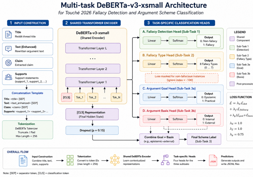
Figure 1: Architecture of the multi-task DeBERTa-v3-xsmall framework.
