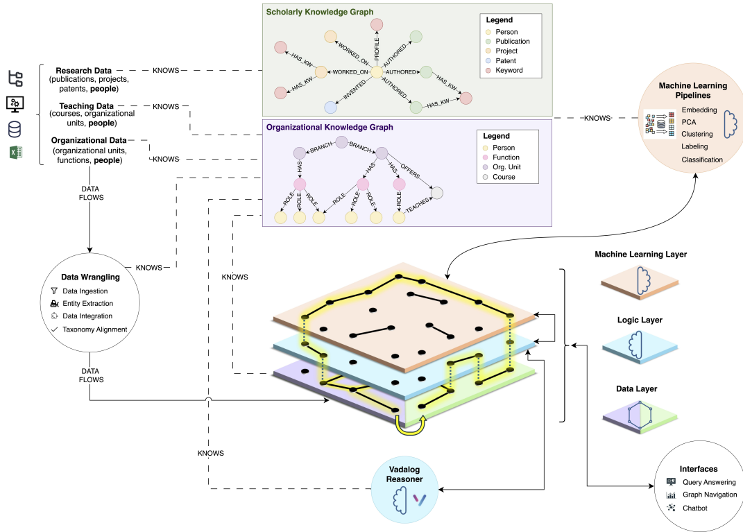
Figure 1: Overview of architecture of the SYNAPSE-KG.
