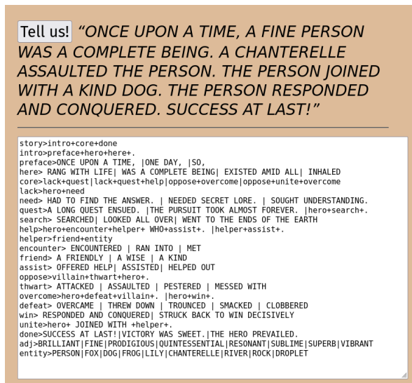
Figure 2: “Gram’s Fairy Tales” with a generated story at the top and the default grammar in a text area below it. The grammar can be edited directly in the browser.
