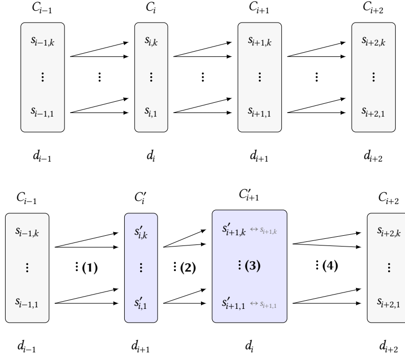
Figure 2: The Sequential Counter on four adjacent columns (top), and the new encoding when swapping d_i and d_{i+1} (bottom). Fresh columns C'_i and C'_{i+1} (blue) replace the originals. In C'_{i+1} , gray suffixes show the equivalences s'_{i+1,j} \leftrightarrow s_{i+1,j} from step (3). In each column gap, the arrows represent the dependencies of the definitions; step numbers (1), (2) add new variables and their defining clauses, whereas step number (4) only adds clauses.
