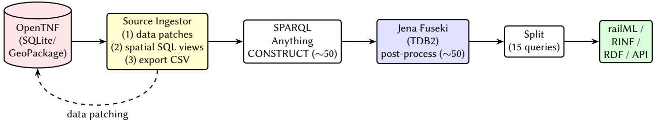
Figure 2: Simplified production pipeline. The Source Ingestor performs data patches and spatial SQL before export; SPARQL Anything maps CSV to RDF; Jena Fuseki hosts the graph and runs post-processing; splitting queries extract subnetworks for railML and RINF export. Orchestration is omitted for clarity.
