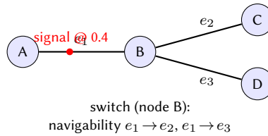
Figure 1: A railway topology as a graph. Node B is a switch connecting edges e_1 , e_2 and e_3 . The signal is positioned by an intrinsic coordinate (0.4) along edge e_1 , not by an absolute point.
