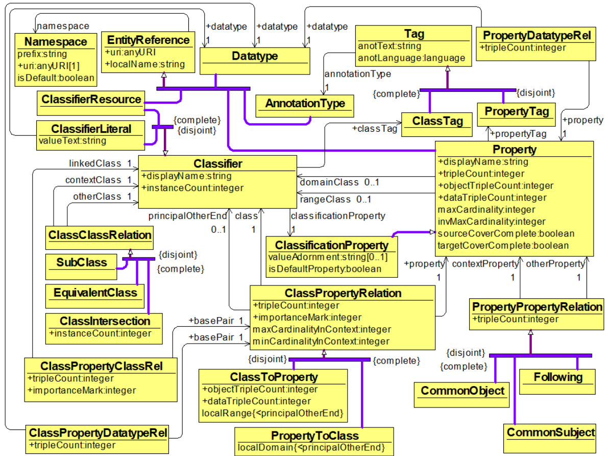
Figure 1: Conceptual data schema structure
