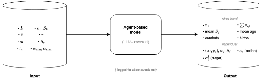
Figure 3: Black-box representation of the simulation model. Input parameters include grid size L , initial population n_0 and sugar S_0 , target average sugar density \bar{s} , vision range v and metabolism m , reproduction threshold S_r , memory length l_m , and genetic mutation parameters \alpha_{min} , \alpha_{max} . At each time step, the model logs step-level statistics (number of alive agents n_t , total map sugar \sum s_{i,t} , mean agent sugar S_j , mean age, cumulative combats, and births) and individual-level data (position, \alpha_j , S_j , action a_j , and, for attack events, the target's \alpha_t ).
