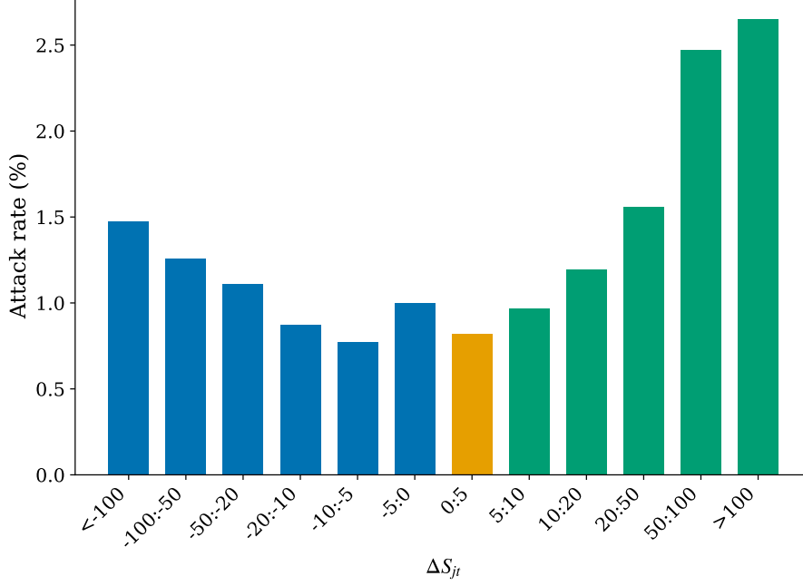
Figure 8: Attack rate (probability of attacking an adjacent agent) as a function of the sugar differential \Delta S_{it} = S_j - S_i between the focal agent and the adjacent neighbor, computed over all adjacency opportunities across all configurations. Bars are colored by sign: blue for \Delta S_{it} < 0 (attacker poorer than target), orange for \Delta S_{it} \approx 0 , green for \Delta S_{it} > 0 (attacker richer). Agents cannot observe the sugar reserves of their neighbors nor the combat mechanic; nevertheless, attack rate increases monotonically with sugar advantage (right side) and shows a secondary increase under large deficit (left side), suggesting emergent strength estimation and desperation-driven aggression respectively.
