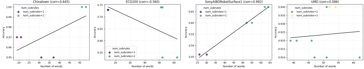
Figure 2: Relation between rule set word count and LLM-proxy accuracy. Each point corresponds to a class-level rule set from one run. The relation is not monotonic: concise rules can be highly effective, but longer rules are not automatically better.
