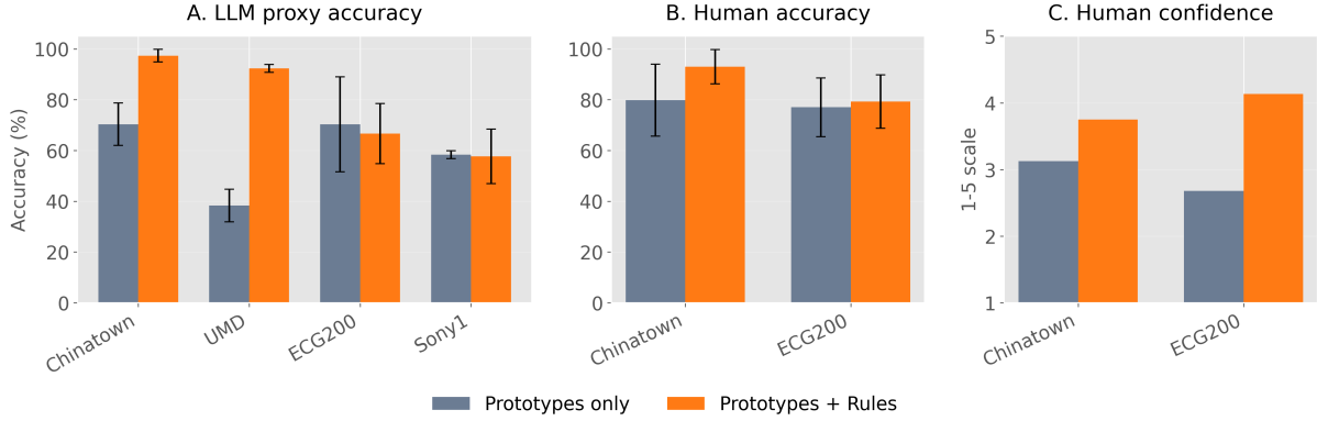
Figure 1: Results overview. Panel A compares LLM proxy forward-simulation accuracy under direct prototype prompting and rule-based prompting. Panels B and C summarise the human study: rules improve classifier-imitation accuracy on Chinatown and increase confidence on both datasets, while ECG200 accuracy changes little, illustrating the dataset-dependency of the verbal translation layer.
