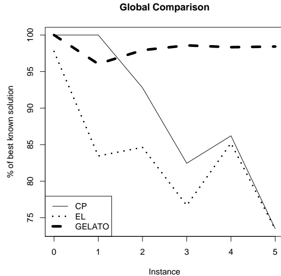
Fig. 2: Comparison of the best solutions obtained by the three methods
