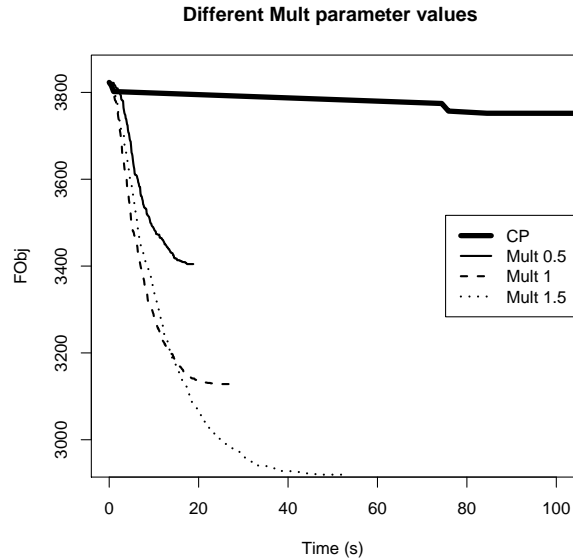
Fig. 4: Comparison between different stop criterions (parameter Mult ) for GELATO
