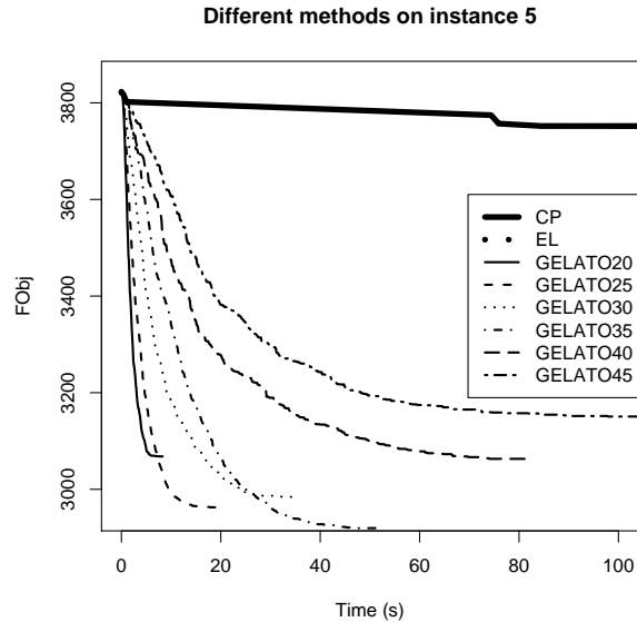
Fig. 3: Comparison between the different approaches on instance 5
