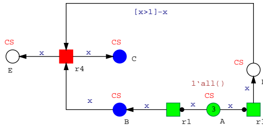
Fig. 3. CPN model for cells linked in a pipeline. The declarations are as follows: colourset CS = \text{int} with 1 - N , variable x: CS . The arc expression [x > 1] - x indicates that the first cell is not linked to the last, meaning cells are linked in a linear pipeline.
